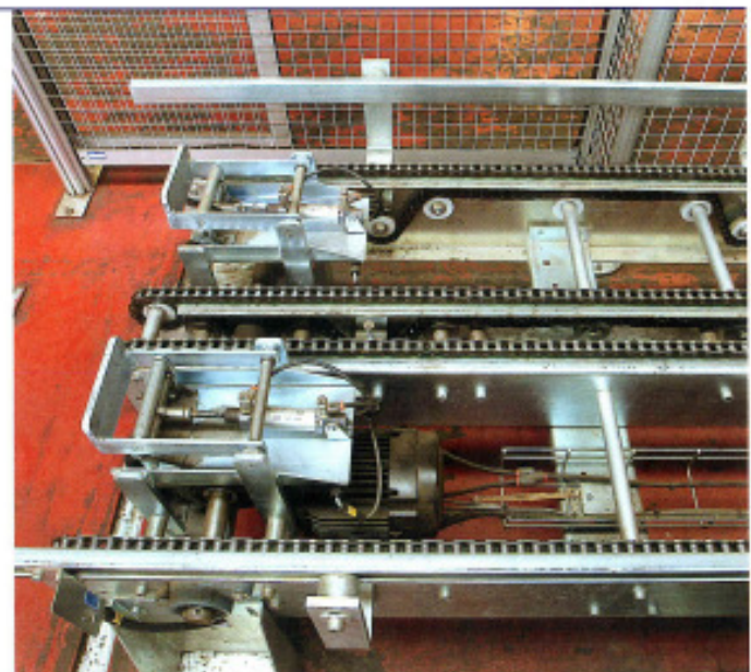
Chain conveyor system for \frac{1}{4} plastic pallets. The system is equipped with pneumatic stops for precise positioning of pallets at Dansk Kaffe Kompagni in Denmark.
