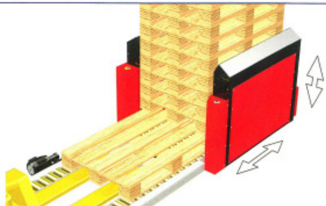
This Multi version stacks/destacks the pallets from pallet roller conveyors of heights as low as 90 mm. Here shown with 2-parted infeed/outfeed conveyor.
